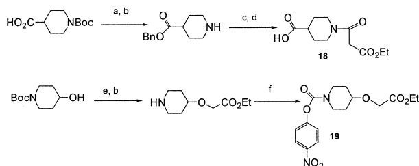
Scheme 5. Synthesis of carboxylic acid segments 18 and 19 . (a) BnOH, DCC, DMAP, DCM; (b) TFA, DCM; (c) ClCOCH 2 CO 2 Et, DIEA, DCM; (d) 10% Pd/C, H 2 ; (e) ethyl diazoacetate, Rh(OAc) 2 -dimer; (f) p -nitrophenylchloroformate, DIEA, DMF.
