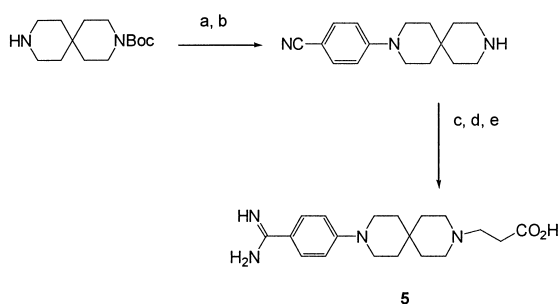
Scheme 2. Synthesis of compound 5 : (a) 4-bromobenzonitrile, \text{Pd}_2(\text{dba})_3\cdot\text{CHCl}_3 , S -BINAP, t -BuONa, toluene, 85 °C; (b) TFA/DCM; (c) \text{Br}(\text{CH}_2)_2\text{CO}_2\text{Et} , DIEA, DCM; (d) LiOH, THF, \text{H}_2\text{O} ; (e) (i) \text{NH}_2\text{OH}\cdot\text{HCl} , \text{Et}_3\text{N} , EtOH; (ii) \text{Ac}_2\text{O} , AcOH, rt; (iii) 1 atm \text{H}_2 , 10% Pd/C, EtOH.
