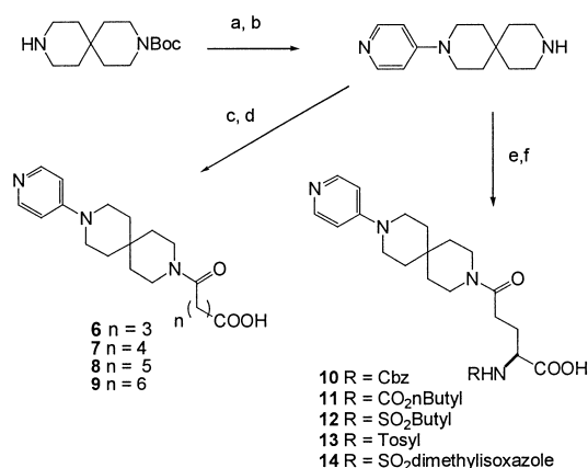
Scheme 3. Synthesis of compounds 6–9 : (a) 4-bromopyridine, \text{Pd}_2(\text{dba})_3\cdot\text{CHCl}_3 , S -BINAP, t -BuONa, toluene, 85 °C; (b) TFA/DCM; (c) \text{ClCO}(\text{CH}_2)_{3-6}\text{CO}_2\text{Et} , DIEA, DCM; (d) 2 M HCl; (e) 20–24 , HOBt, DIEA, DMF; (f) 2 M HCl.
