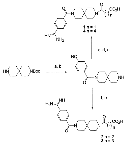
Scheme 1. Synthesis of compounds 1–4 : (a) 4-cyanobenzoyl chloride, TEA, DCM, DMAP; (b) TFA/DCM; (c) \text{ClCO}(\text{CH}_2)_{1,4}\text{CO}_2\text{Et} , TEA, DCM; (d) 1 N NaOH; (e) (i) \text{H}_2\text{S} , \text{Et}_3\text{N} , Pyr; (ii) MeI, acetone, rt; (iii) \text{NH}_4\text{OAc} , EtOH, reflux; (f) succinic or glutaric anhydride, \text{Et}_3\text{N} , DCM.
