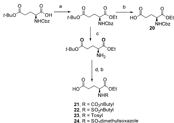
Scheme 6. Synthesis of carboxylic acid segments 20–24 . (a) EDC, HOBT, EtOH; (b) TFA, DCM; (c) Pd(OH) 2 , 1 atm H 2 , EtOH; (d) RSO 2 Cl or ROCOCl, DIEA, DMF.
