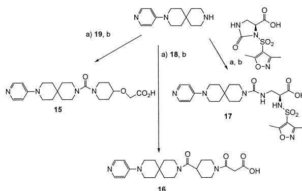
Scheme 4. Synthesis of compounds 15–17 : (a) DMF, DIEA, 60 °C, DMF; (b) 2 M HCl.
